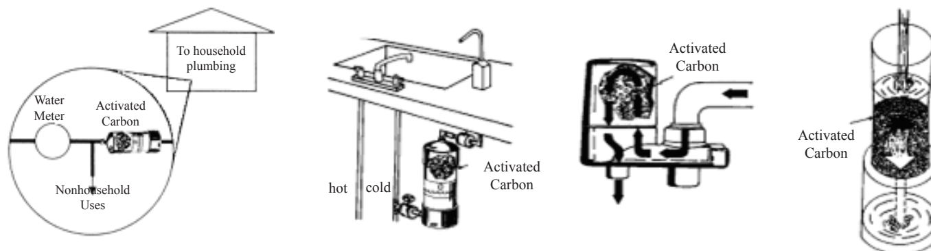
Figure 2. Types of activated carbon filtration units are: (from left to right) Point of entry, line bypass, faucet-mounted, and pour through. Adapted from "Treatment Systems for Household Water Supplies: Activated Carbon Filtration," North Dakota State University Extension Service.
